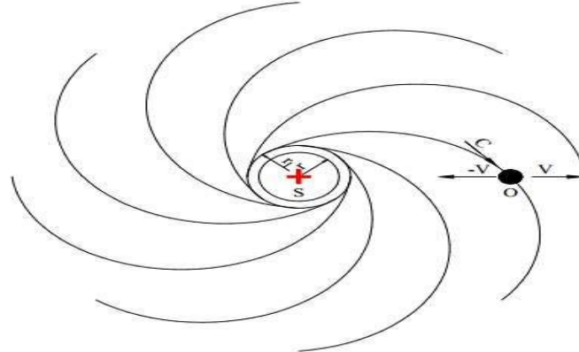
Fig. 1. S - light source (the atom), O - observer, r - radius of the atom, r_1 - the radius of the orbit of the highest flux at his address in a calm state, prior to heating (at orbital velocity), v - relative velocity of removal or approximation between S and O, c - velocity of light vector.
