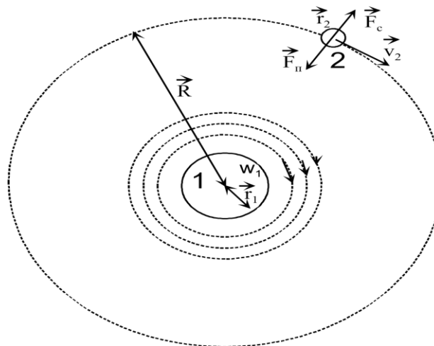
Fig.1. Two-dimensional model of the gravitational interaction between the two bodies.
