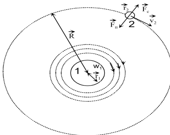
Fig. 1. Two-dimensional model of gravitational interaction of two bodies. Forces operating on a body 2 are specified. The F_c -centrifugal force, F_p -force of an attraction of a body 2 from a body 1, v_2 – the linear speed of a body 2 on an orbit, R – the radius of an orbit, r_1 – the radius of a body 1, r_2 – the radius of a body 2, w_1 – the angular speed of rotation of air on a surface of a body 1, m_2 – body weight 2.
