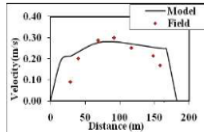
Fig. 9. Flow velocity calibration at cross section (3)
