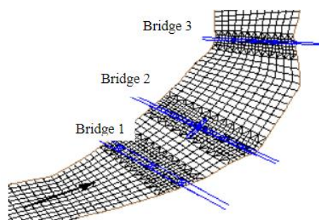
Fig. 5. Mesh generation
