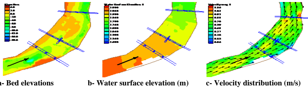
Fig. 13. The procedures of applying the 2-d model on the Kafr El-Zayat bridges at maximum flow conditions
