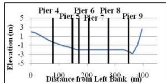
Fig. 16. Second bridge piers location
