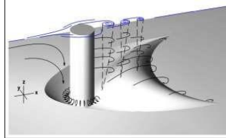
Fig. 2. Flow profile around a circular bridge pier
