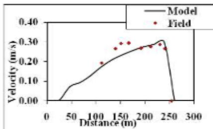
Fig. 8. Flow velocity calibration at cross section (2)
