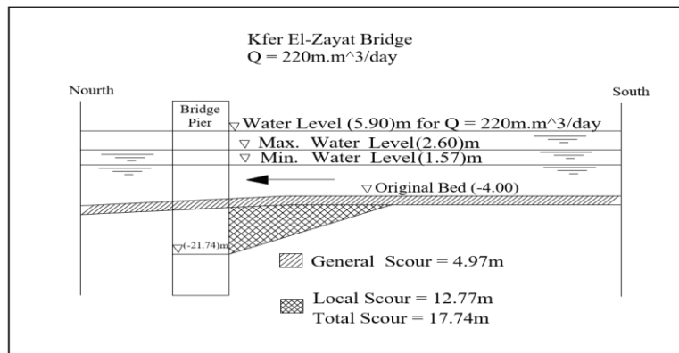
Fig. 14. Evaluation of the total scour at Kafr El-Zayat
