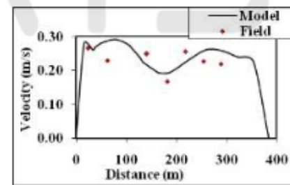
Fig. 7. Flow velocity calibration at cross section (1)
