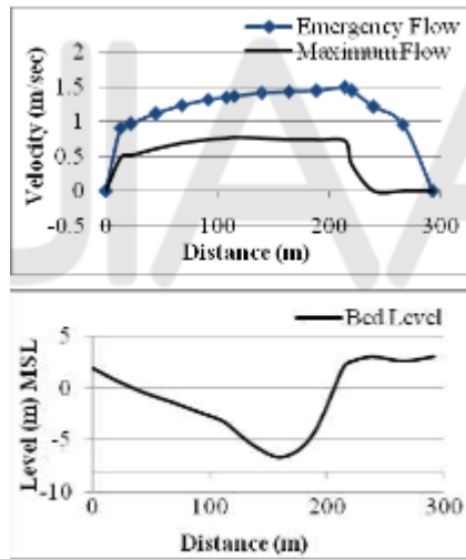
Fig.10.The velocity and bed profile at cross section a in cases of maximum and emergency flow
