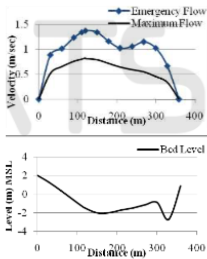
Fig.11.The velocity and bed profile at cross section b in cases of maximum and emergency flow
