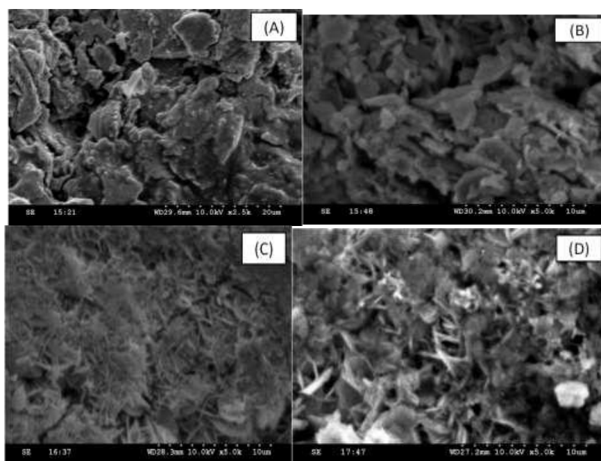
Figure 6: SEM images of aluminium coupons in 0% (A); 10% (B); 30% (C) and 50% (D) Azadirachta indica leaf extract in 1.85 M HCl solution
