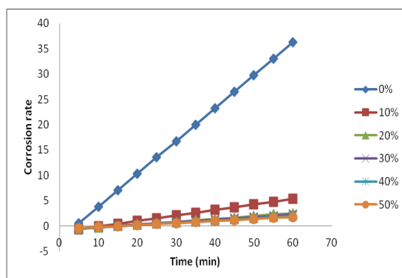
Fig. 4: Corrosion rate of varying concentrations of Azadirachta indica extract with time (min) on Aluminium coupon in 1.85 M HCl solutions at room temperature.
