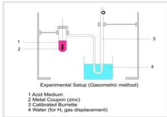
Figure 1: Experimental set up for gasometric method
