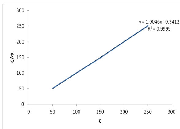
Figure 5: Langmuir adsorption plot for aluminium corrosion in Azadirachta indica extract in 1.85 M at 15 min.
