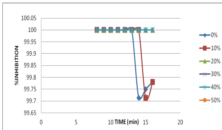
Figure 3: Percentage inhibition efficiency of varying concentration of Azadirachta indica extracts with time on Aluminium coupon in 1.85 M HCl solution at room temperature.
