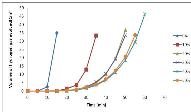
Figure 2: Variation of volume of hydrogen ( \text{cm}^3 ) evolved with time (min) of Aluminium coupons for different concentration of Azadirachta indica extract in 1.85M HCl at room temperature.
