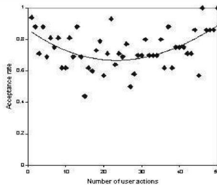
Figure 3: Performance of Stock Tracker with human subjects in terms of acceptance rate.
