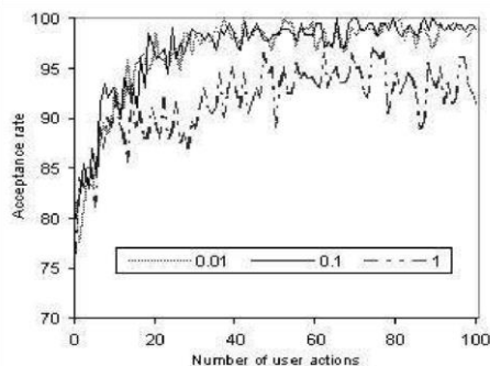
Figure 6: Acceptance rate for Stock Tracker recommendations with different default model weights.
