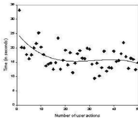
Figure 4: Performance of Stock Tracker with human subjects in terms of time spent on each transaction.
