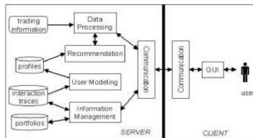
Figure 1: Architecture for the Stock Tracker.
