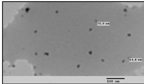
Fig. (2): Transmission Electron Microscopy (TEM)
