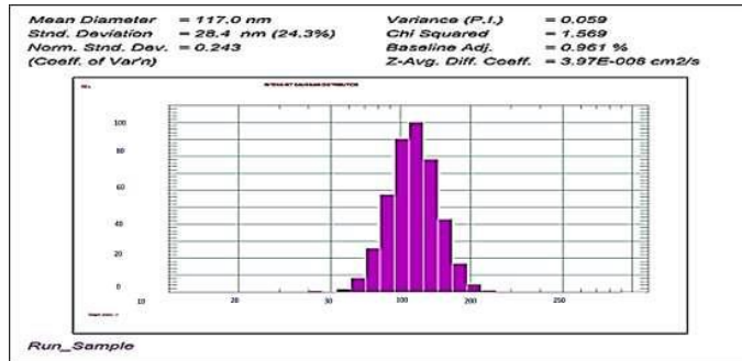
Fig. (1): Dynamic light scattering measurement (DLS)
